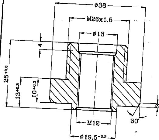
part 1 Welding piece St37-2
