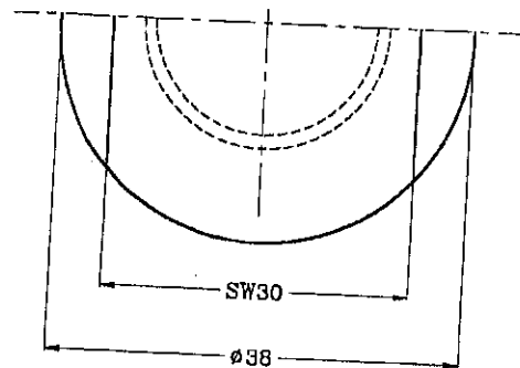
part 2 cap nut St37-2
